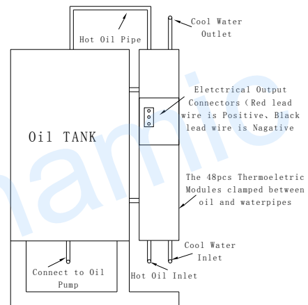
500W- 48VDC Output Thermoelectric Generator Diagram
