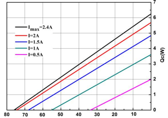
The chart for Q_c Vs DT under various currents
